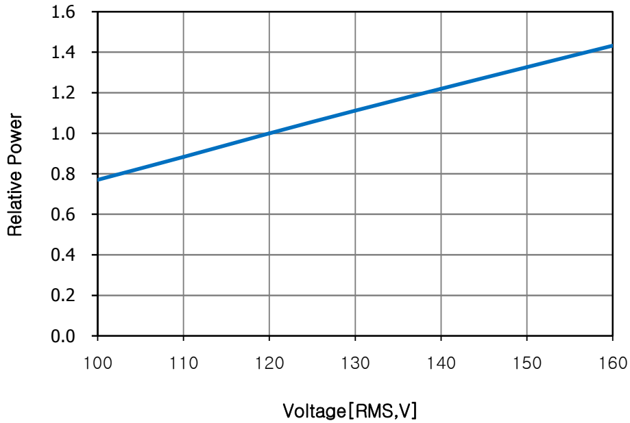
Fig 4. Relative Power Distribution vs. Voltage, T_a=25^\circ\text{C} , 120V
